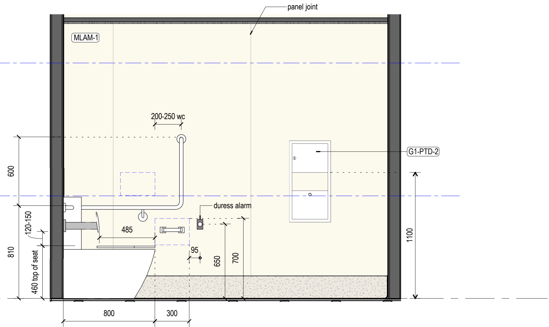
3 0.14 - PWD - East Elevation 1 : 20
