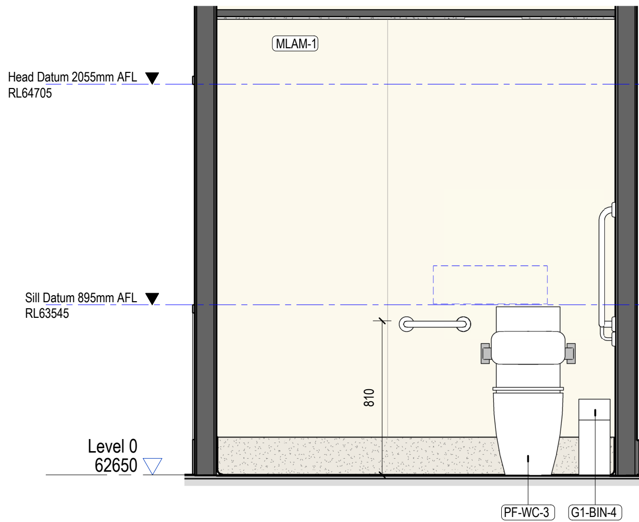
4 0.14 - PWD - North Elevation 1 : 20
